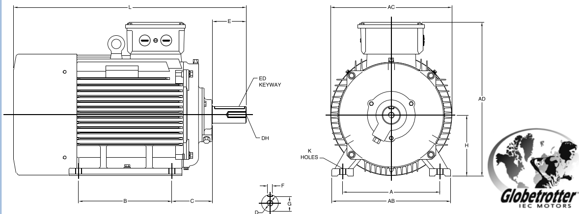
IEC Frame Dimensions (Millimeters)
